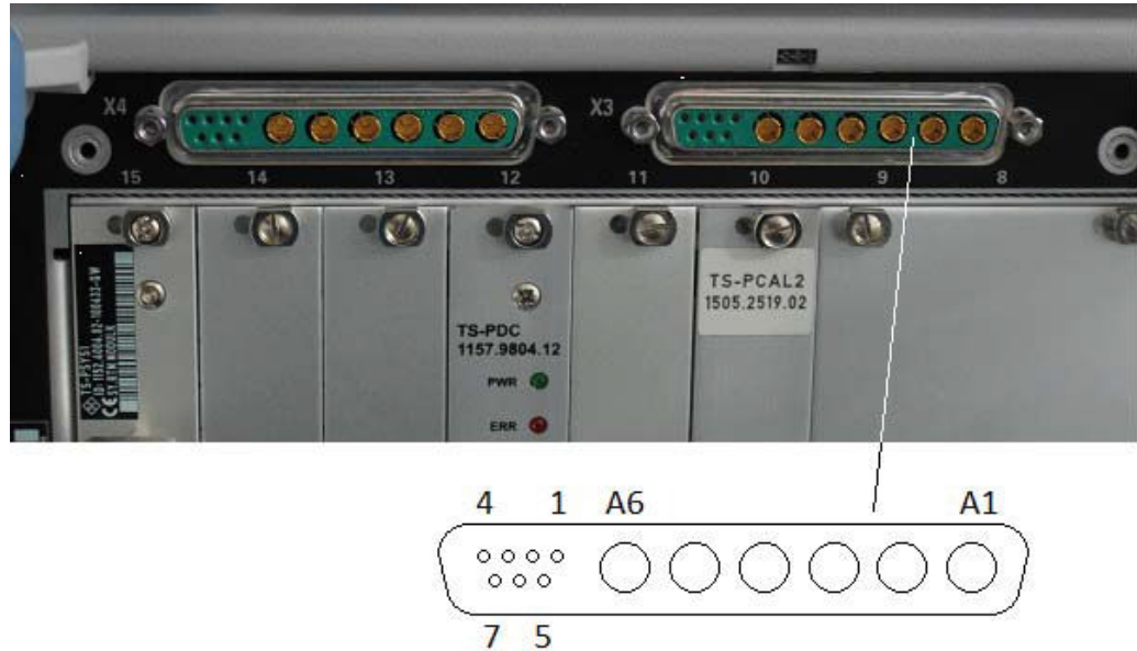
Figure 9-8: Connector X3 - Rear Side R&S TS-PCA3 or R&S TS-PWA3
