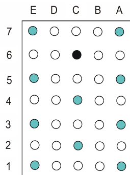
Figure 9-7: Connector X30 (mating side)
