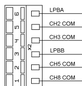
Figure 9-2: Terminal X2
