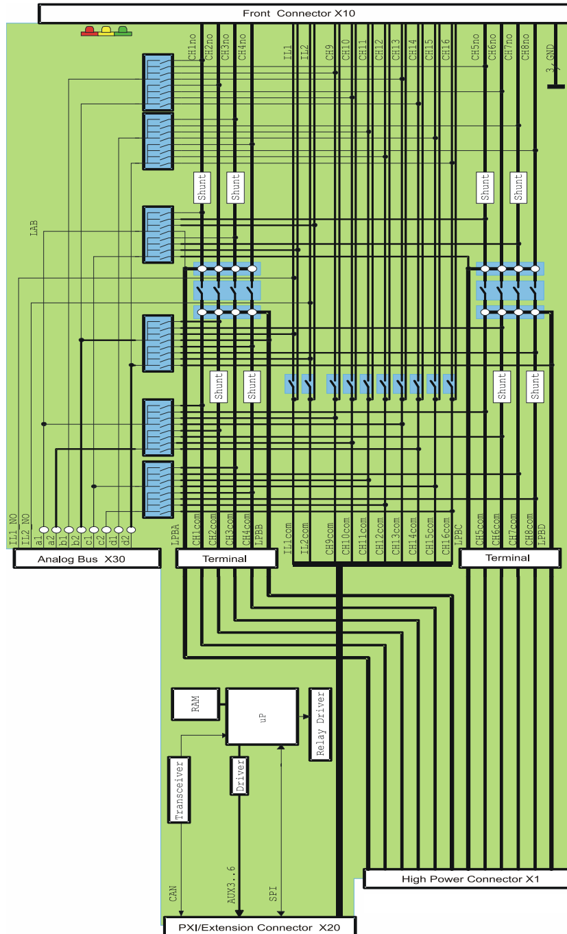
Figure 3-1: Block Diagram R&S TS-PSM1
