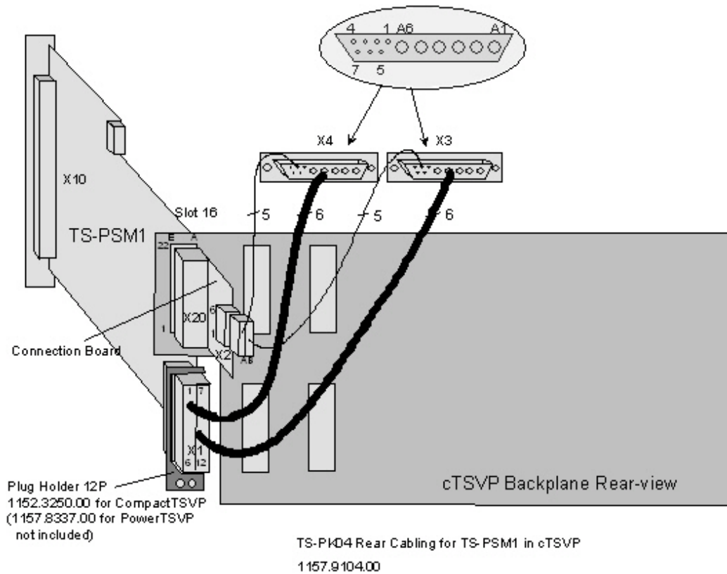
Figure 4-3: R&S TS-PK04 Installation in R&S TS-PCA3 (cTSVP)
