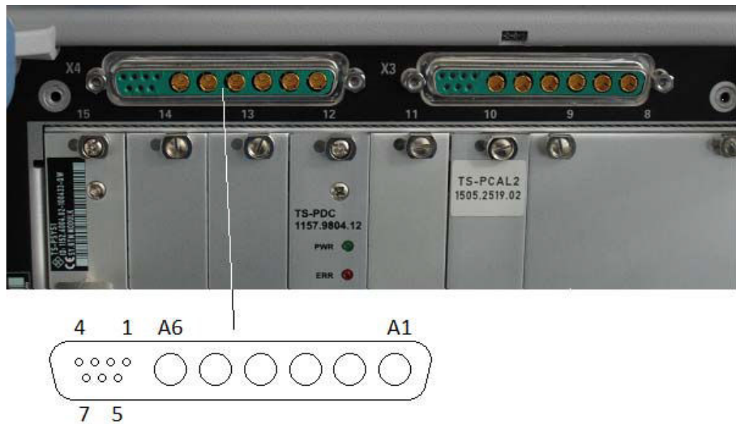
Figure 9-9: Connector X4 - Rear Side R&S TS-PCA3 or R&S TS-PWA3
