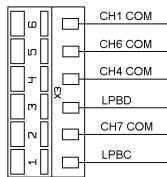
Figure 9-3: Terminal X3
