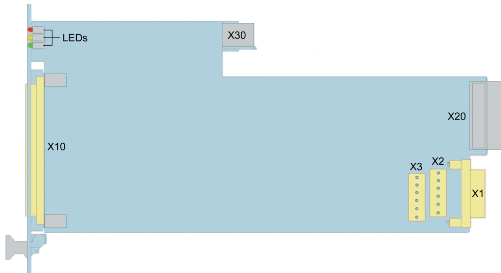
Figure 4-1: Layout of Connectors and LED's
