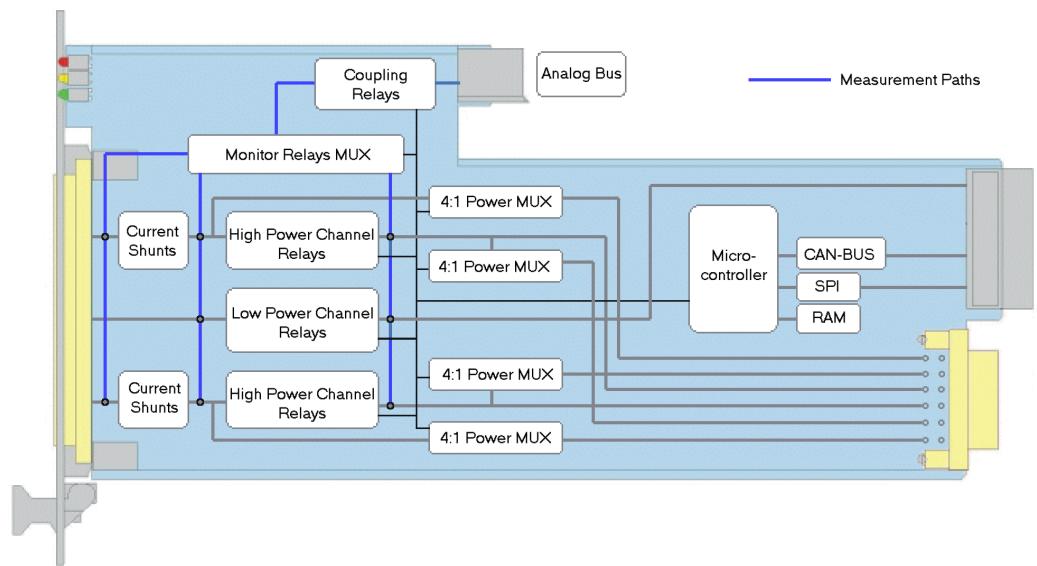
Figure 3-2: Functional Block Diagram R&S TS-PSM1
