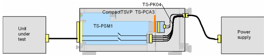
Figure 4-2: Installation of R&S TS-PSM1 with R&S TS-PK04 in the CompactTSVP R&S TS-PCA3
