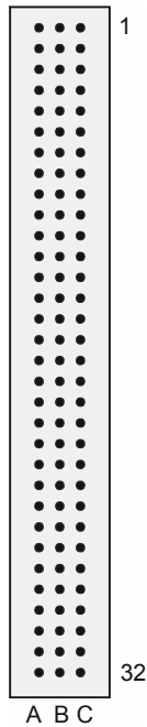
Figure 9-4: Connector X10 (mating side)
