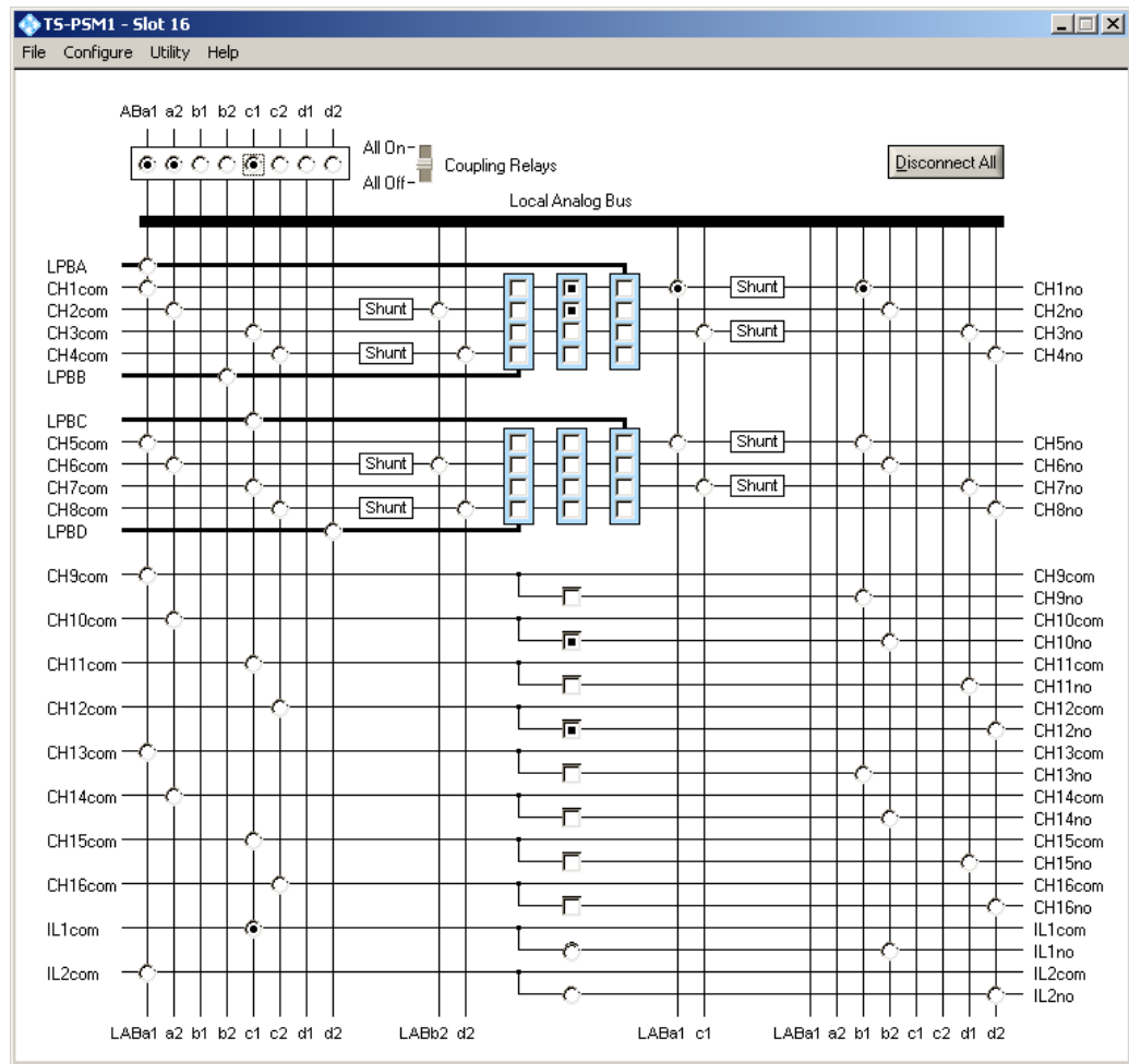
Figure 7-1: Softpanel R&S TS-PSM1
